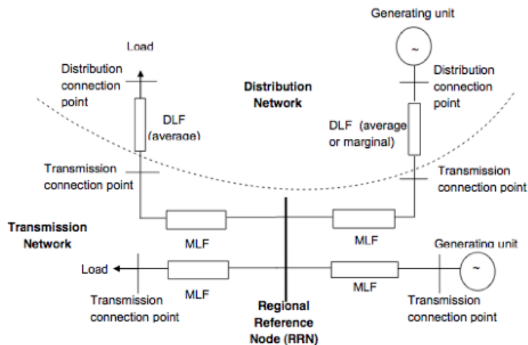
Figure 5-16: Relationship between connection points and loss factors (AEMO, 2009)
