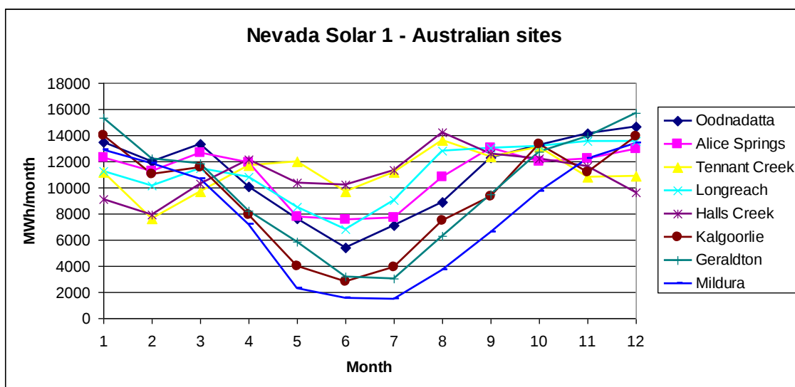
Figure 5-2: Modelled outputs of a parabolic trough system at various Australian sites
