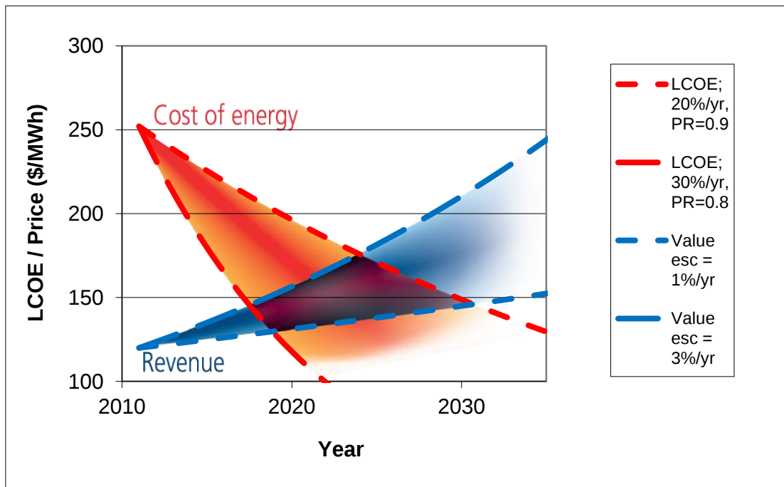
Figure 6-22: Possible progression of indicative CSP LCOE and market value in Australia (2011 real AUD)
