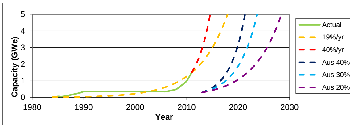
Figure 8-1: Global CSP development trajectories and projections, as well as possible Australian trajectories, if the same percentage growth profiles are followed. (Capacity normalised to a 20 -30% capacity factor)
